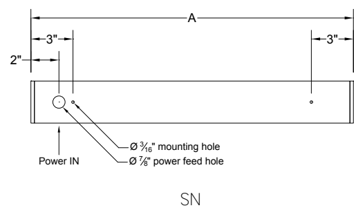
Back Plan - Surface Mount Single Fixture Option
