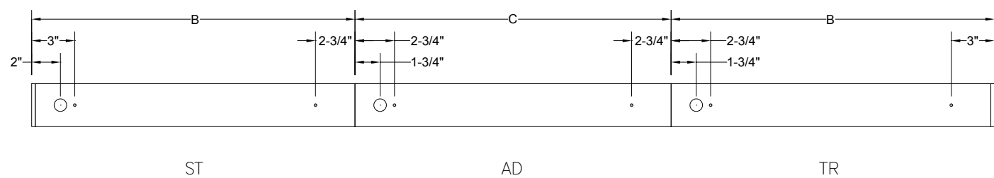
Back Plan - Surface Mount Continuous Run Option
