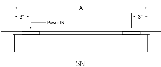
Plan - Wall Mount Single Fixture Option
