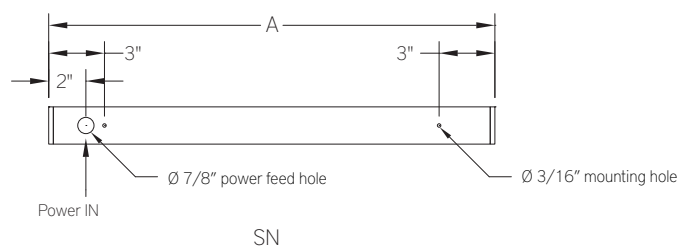
Back Plan - Surface Mount Continuous Run
