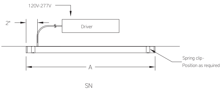
Side View - S1 Surface Mount Single Fixture
