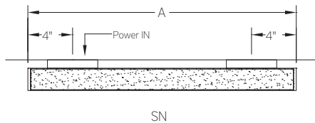
Plan - Wall Mount Single Fixture
