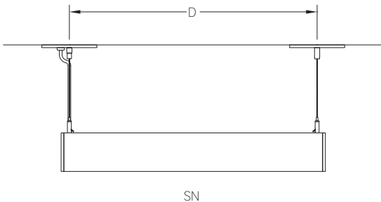
Side View- Cable Suspended Continuous Run
