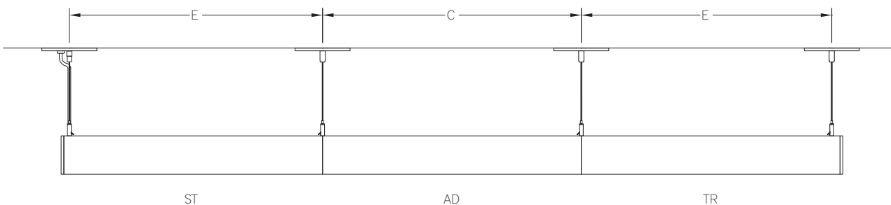
Side View- Cable Suspended Continuous Run
