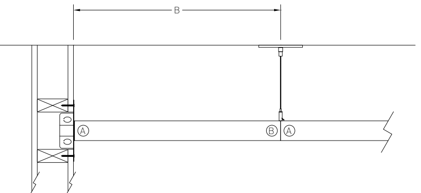
Continuous Fixture Interface with Wall Plate
