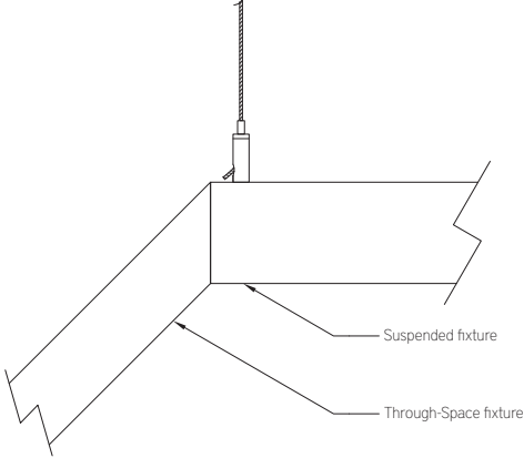
Mounting to BFZ100-S suspended fixture
