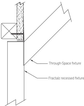
Mounting to BFZ100-R recessed fixture
