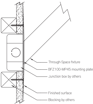
Mounting to BFZ100-MP45 accessory mounting plate
