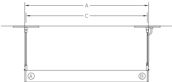
Continuous Fixture Interface with Suspended
