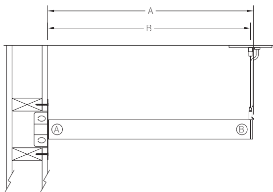
Single Fixture Interface with Wall Plate
