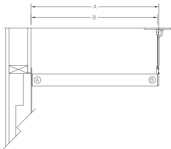
Single Fixture Interface with Recessed
