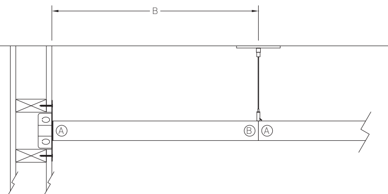
Continuous Fixture Interface with Wall Plate
