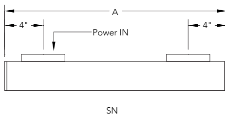
Plan - Wall Mount Single Fixture Option
