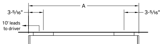
Plan - Wall Mount Single Fixture Option
