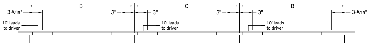
Plan - Wall Mount Continuous Run Option
