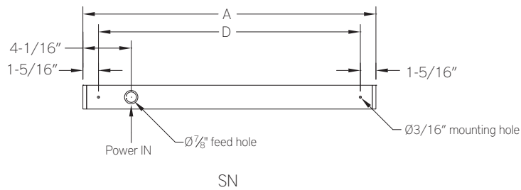
Back Plan - Surface Mount Continuous Run Option
