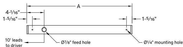
Back Plan - Surface Mount Single Fixture Option
