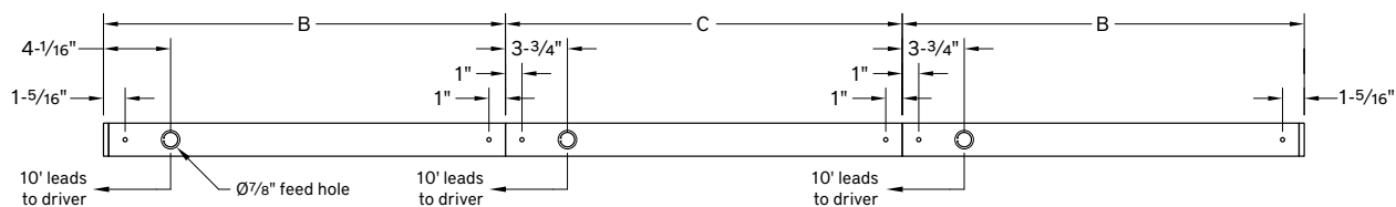
Back Plan - Surface Mount Continuous Run Option
