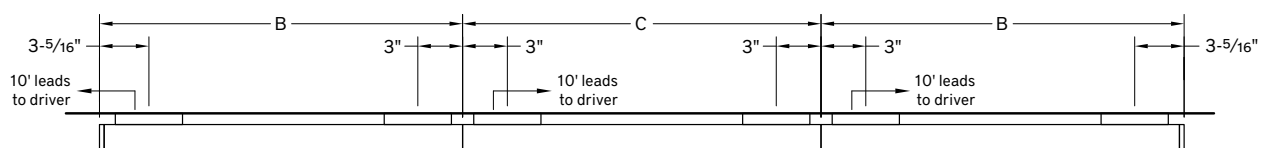
Plan - Wall Mount Continuous Run Option
