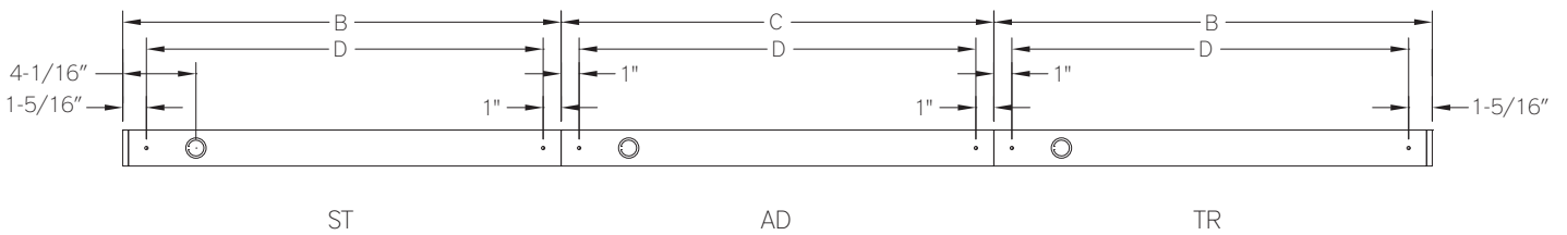
Back Plan - Surface Mount Continuous Run Option
