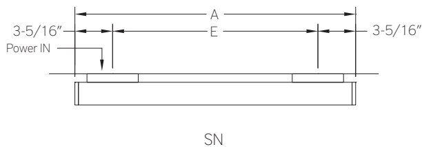
Plan - Wall Mount Continuous Run Option
