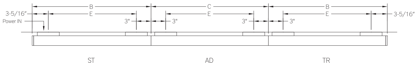
Plan - Wall Mount Continuous Run Option
