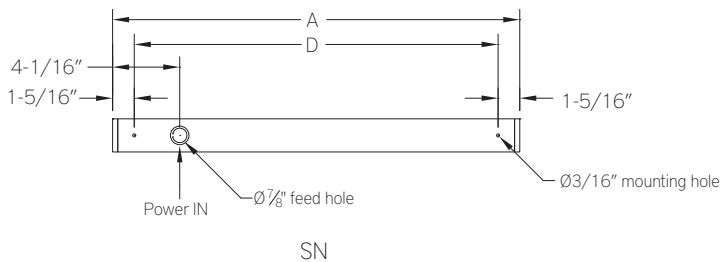
Back Plan - Surface Mount Single Fixture Option
