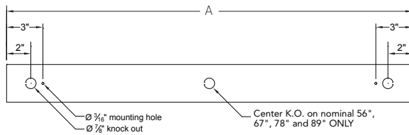
Back Plan - Surface Mount Single Fixture Option
