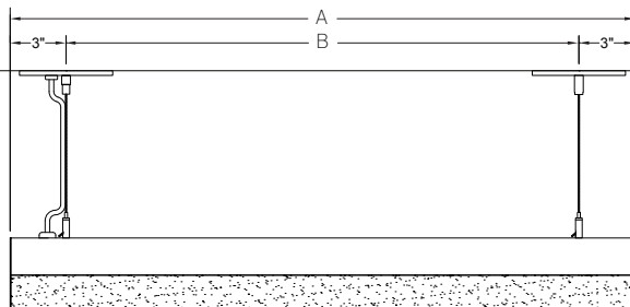
Side View - Cable Mount Single Fixture Option
