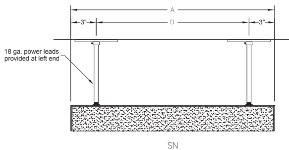
Side View - Pendant Mount Single Fixture Option
