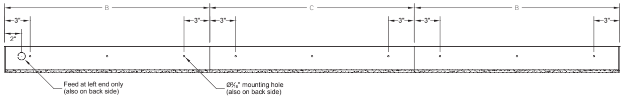
Front View - Surface Mount Continuous Fixture Option
