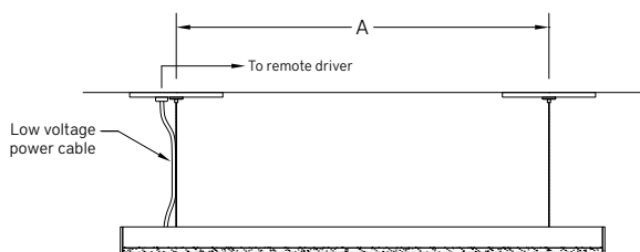
Side View - Cable Mount Single Fixture Option
