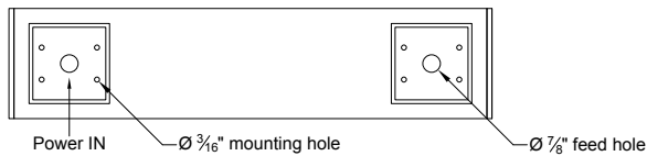
Rear View - Wall Mount Single Fixture Option
