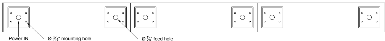
Rear View - Wall Mount Continuous Run Option
