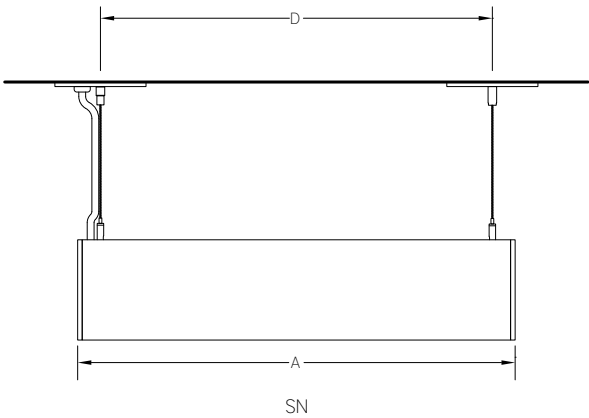
Side View - Cable Suspended Single Fixture
