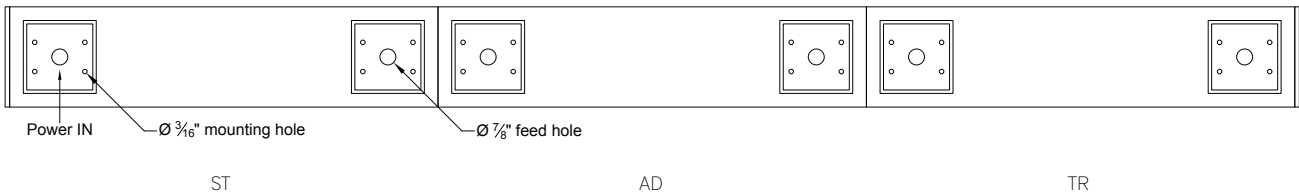
Rear View - Wall Mount Continuous Run Option
