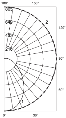
#1 - Vertical plane through horizontal angles (0-180) (through max cd) #2 - Horizontal cone through vertical angle (0) (through max cd)
